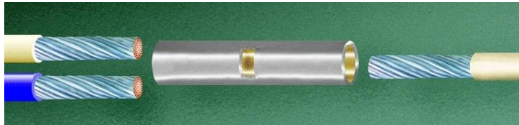
Figure 19-28. Butt Splice Prior to Wire Insertion
