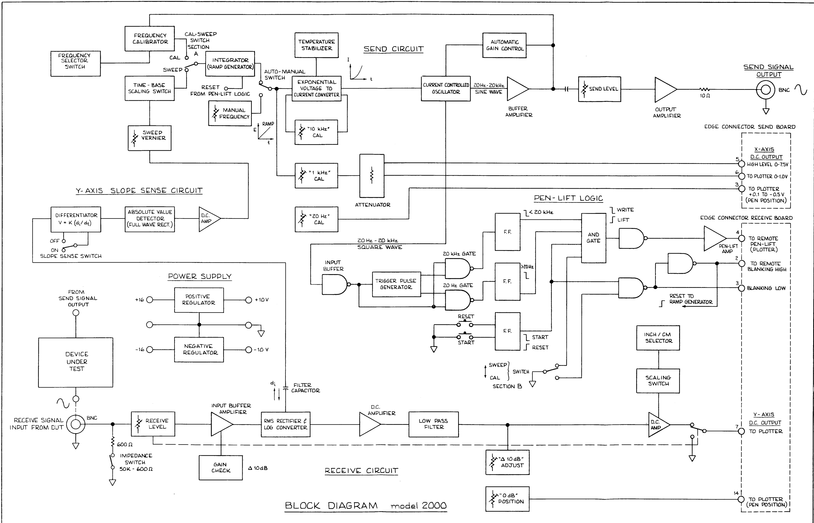
FIG 2 BLOCK DIAGRAM model 2000
