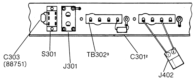
VIEW B-B
