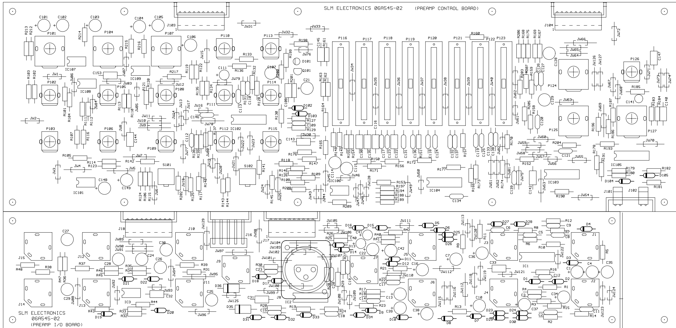
ASSY PART # 07-545-02
