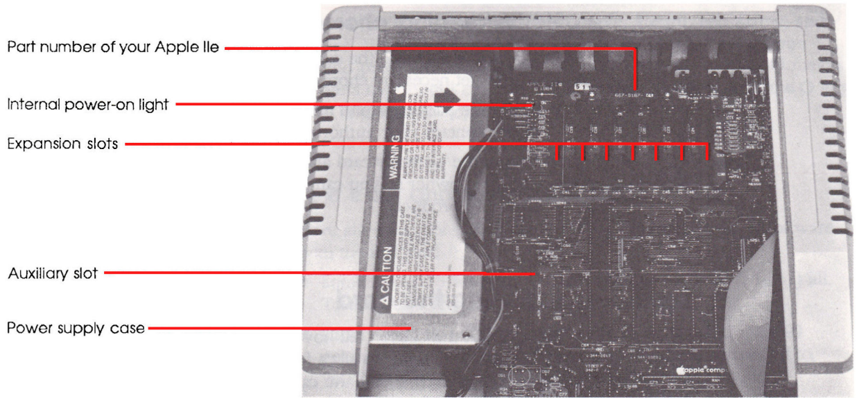
Figure 1 The inside of the Apple IIe
