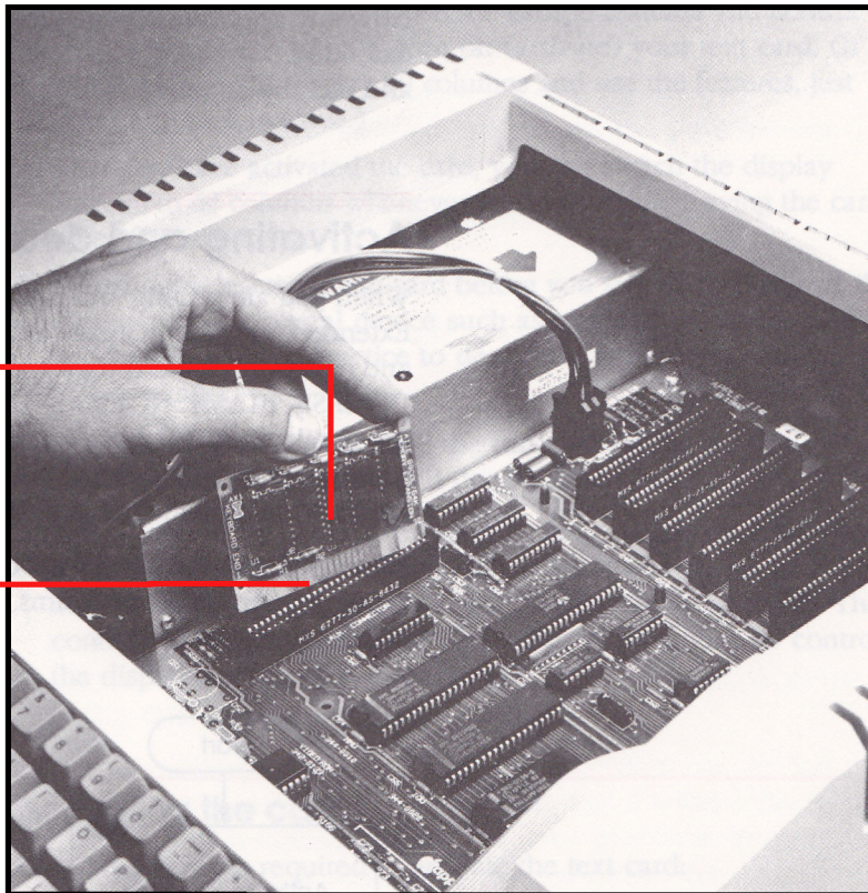
Figure 3 The correct card position
