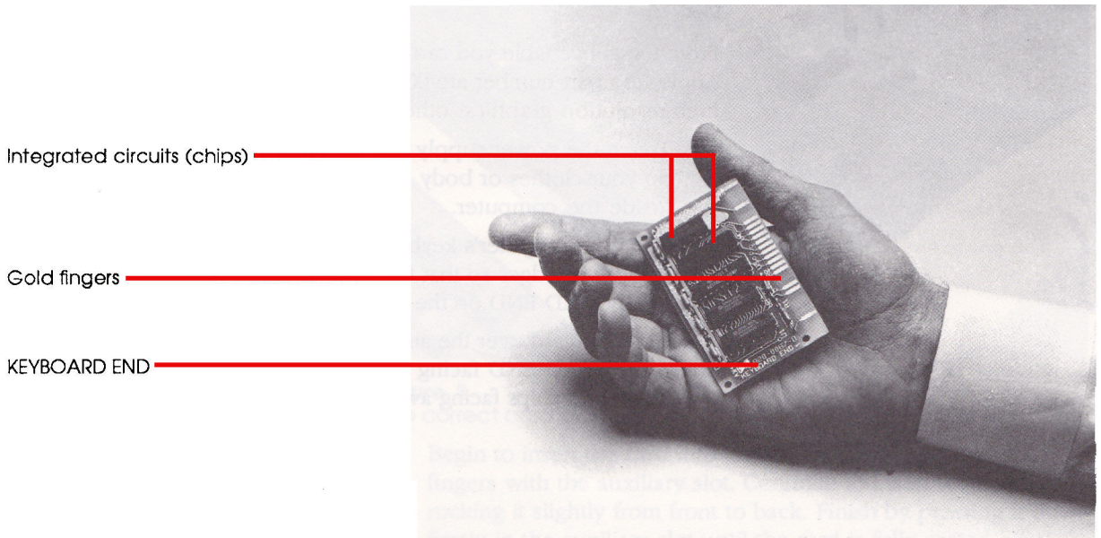
Figure 2 The Extended 80-Column Text Card
