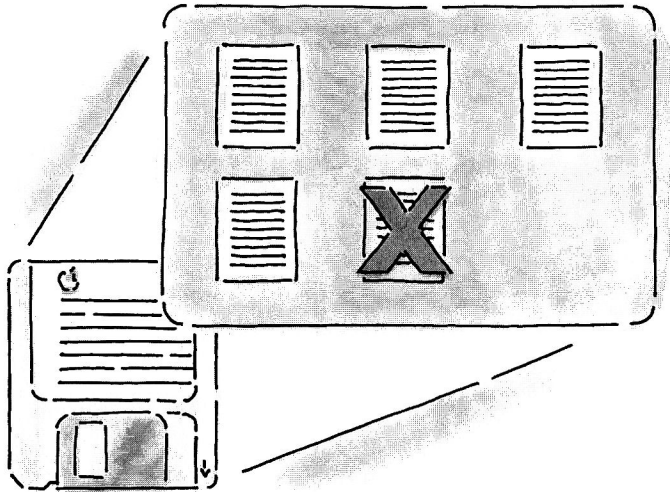
Figure 5-4 Deleting files
