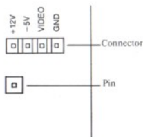
Figure 15. Auxiliary Video Output Connector and Pin.
