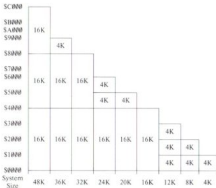
Figure 6. Memory Configurations
