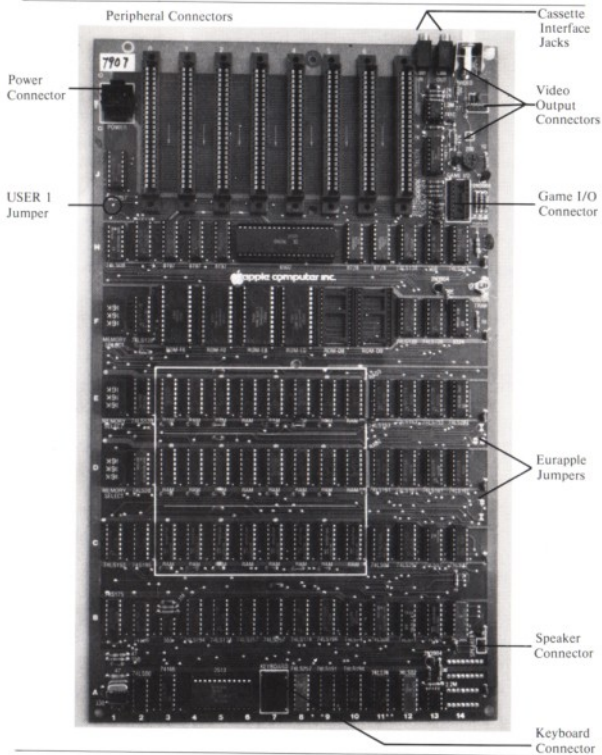
Figure 10. The Apple Main Board
