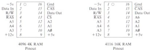
Figure 14. RAM Pinouts
