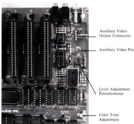
Photo 4. The Video Connectors and Potentiometer.
