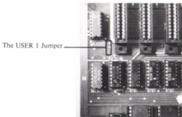
Photo 8. The USER 1 Jumper.
