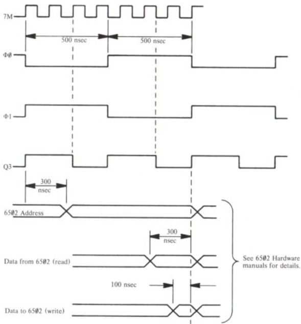
Figure 11. Timing Signals and Relationships
